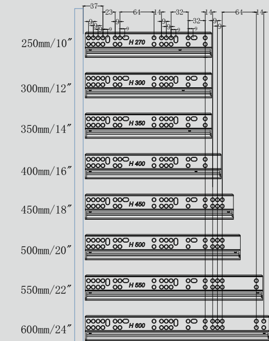
侧孔图 Drill Pic.
