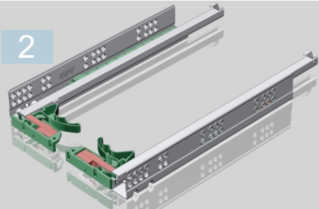
侧孔图 Drill Pic.
