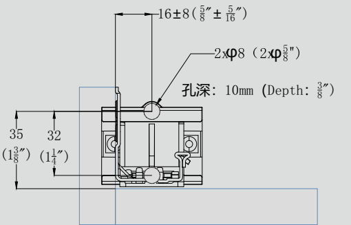
6 背板打孔 Drilling
