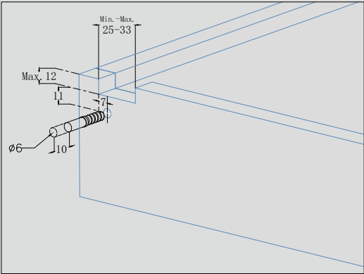
6 抽屉打孔 Drilling
