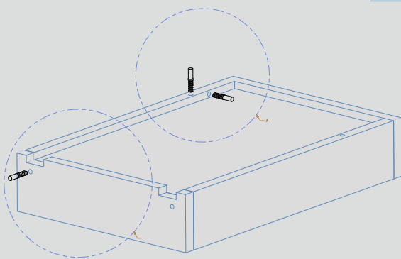
抽屉打孔 Drilling
