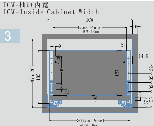
抽屉宽示意图 Cabinet Width Installation.
