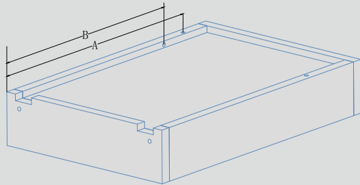
5 抽屉侧孔-距离 Drilling Distance
