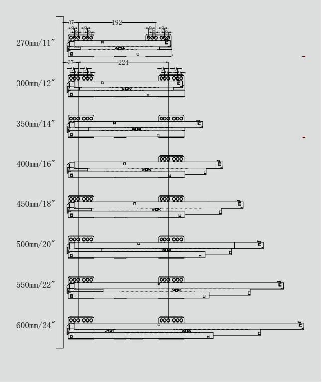
侧孔图 Drill Pic.
