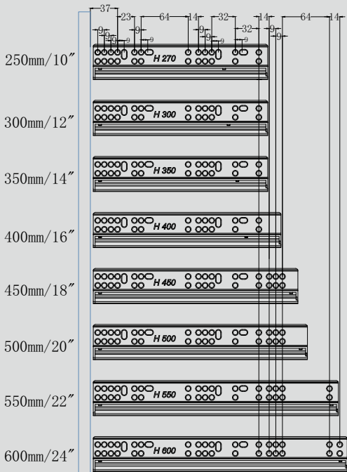
侧孔图 Drill Pic.
