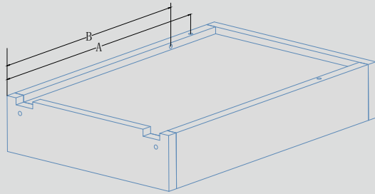
5 抽屉侧孔-距离 Drilling Distance
