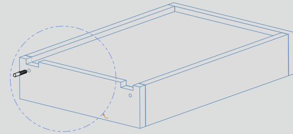
5 抽屉测孔-距离 Drilling Distance
