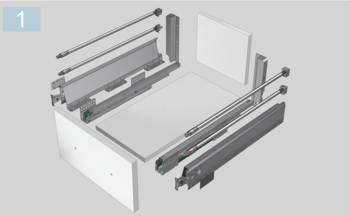
产品图 Products Pic. 产品描述: Product Dia.
