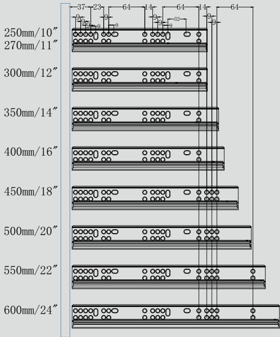
侧孔图 Drill Pic.
