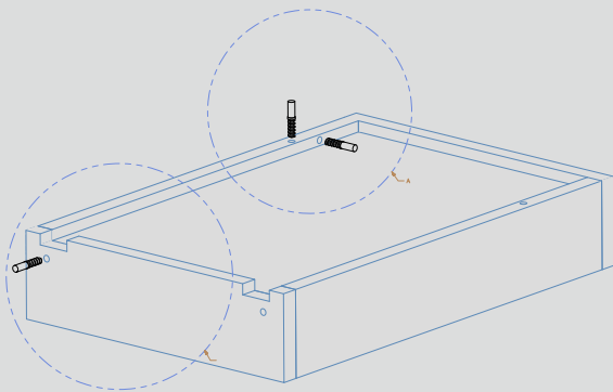
6 抽屉打孔 Drilling
