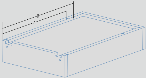
5 抽屉测孔-距离 Drilling Distance
