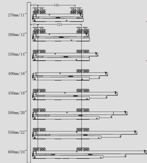
侧孔图 Drill Pic.
