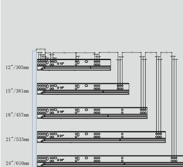
侧孔图 Drill Pic.
