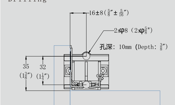
背板打孔 Drilling
