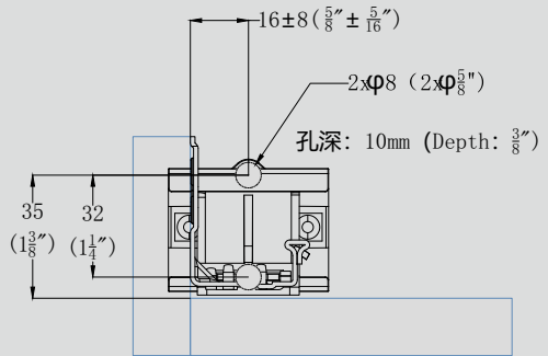
背板打孔 Drilling
