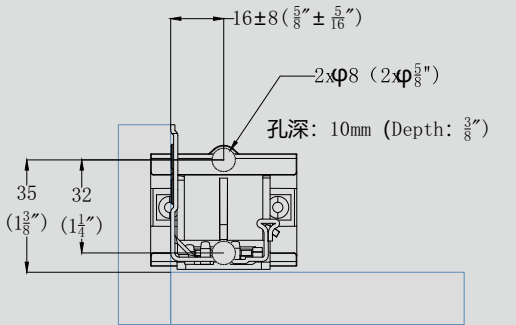
6 背板打孔 Drilling
