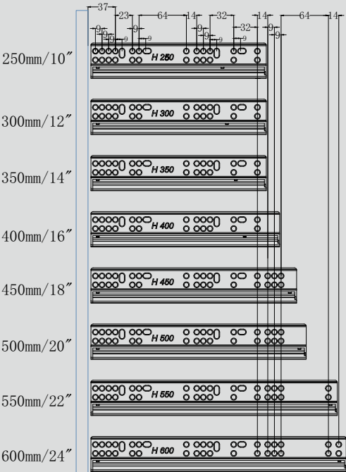
侧孔图 Drill Pic.
